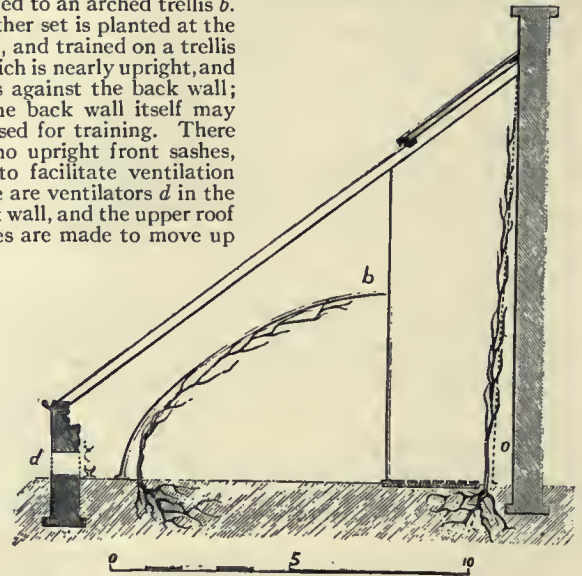
FIG. 8.—Peach House.
